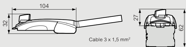
Conector 10 A
